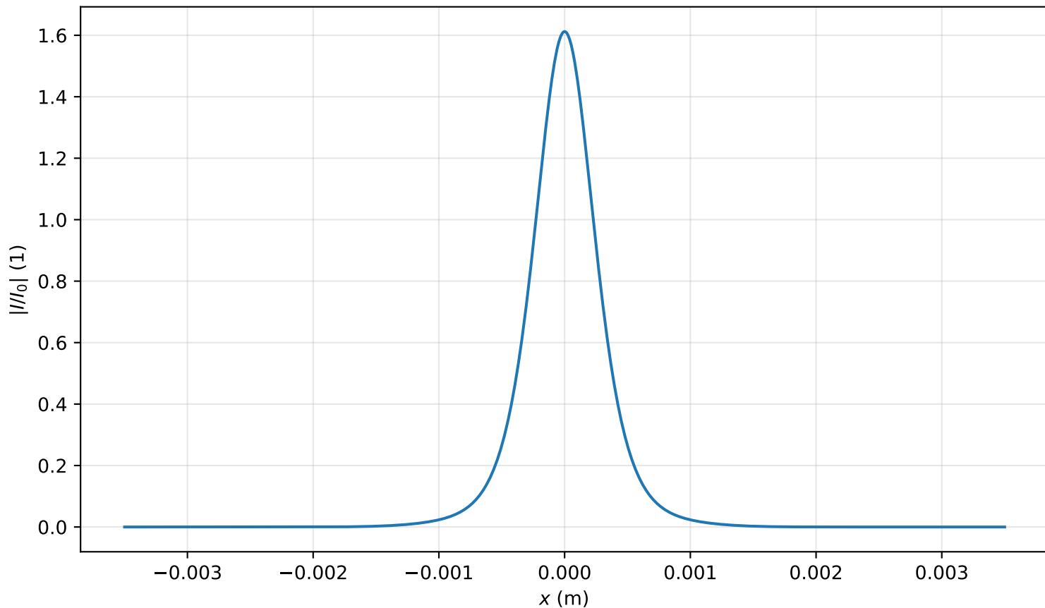
Intensity profile I(x, y = 0, z = 1.751m)/I_0 , P_{in}=0.9P_{cr} , artificial time
